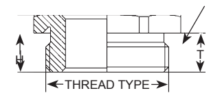
Nickel Plated Brass Hex Plug
